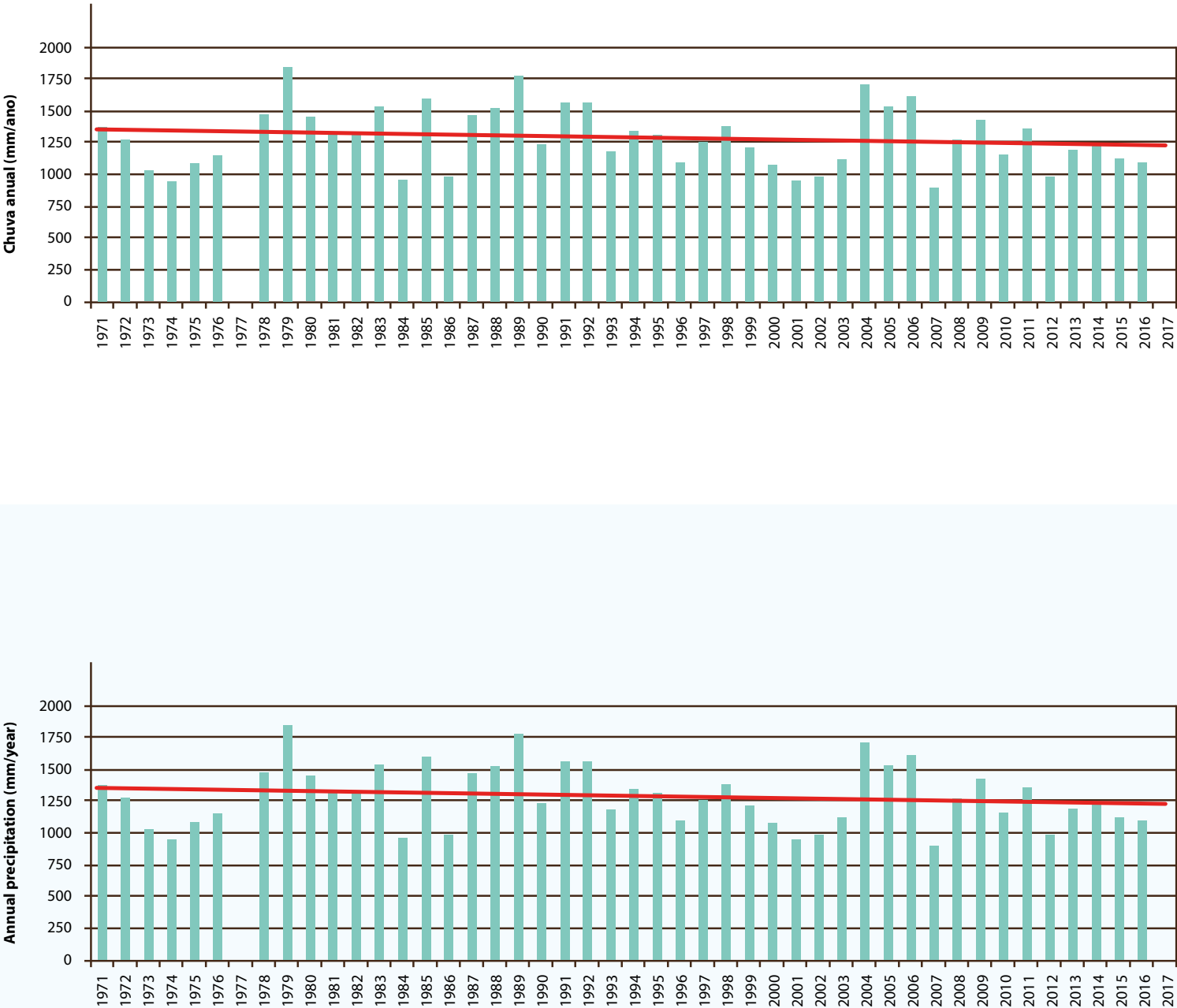
Figure 5. Time series of annual total precipitation in the Taquara station and data trend
