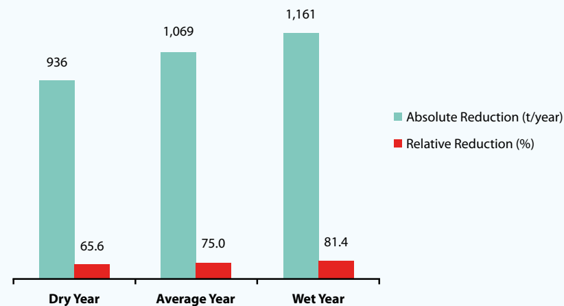
Figure 6. Estimate of the reduction in the transportation of sediments to the basin's mouth after full deployment of the PPA Source: Chaves, 2012.
