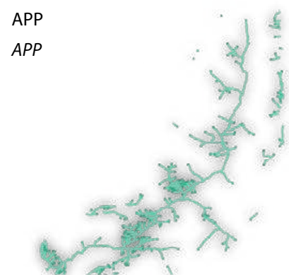
Figure 3. Data layers, updated or mapped using ALOS images for the Pipiripau River Basin, DF
