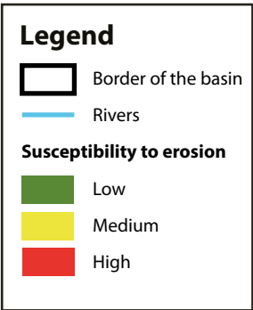
Figure 4. Map of susceptibility to erosion of the Pipiripau river, in 30 m cells Source: Lima et al., 2013b.
