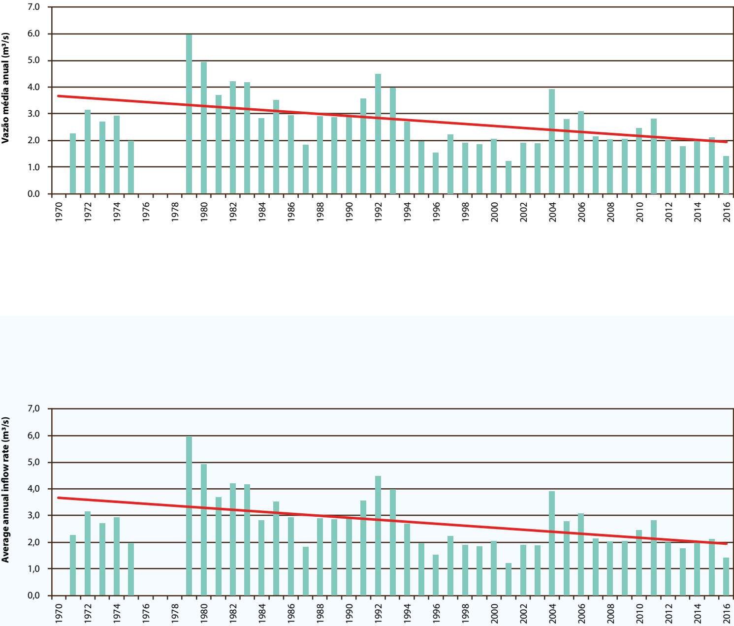
Figure 2. Time series of average annual inflow rate at the Pipiripau Frinocap DF-130 station and data trend
