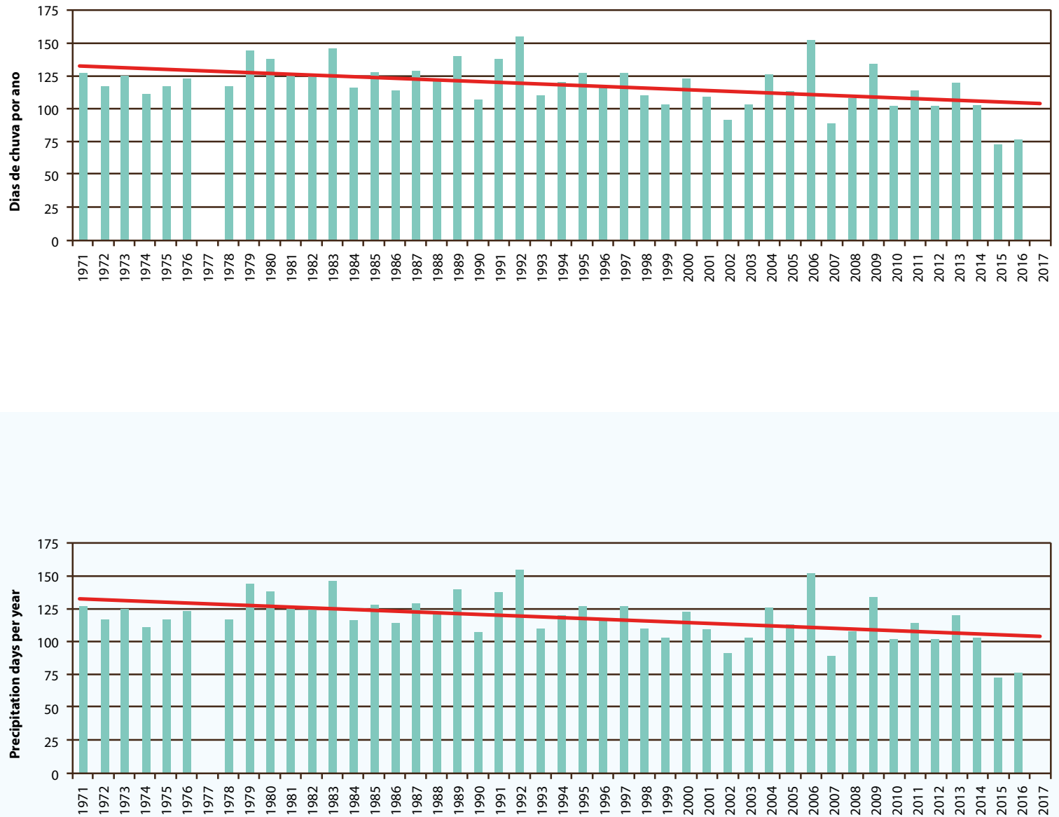
Figure 8. Time series of precipitation days per year in the Taquara station and data trend |
